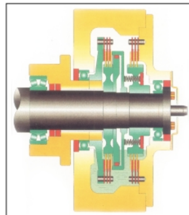
HIGH TORQUE WET CLUTCH & BRAKE UNIT WITH SINTERED MULTI DISC LININGS
