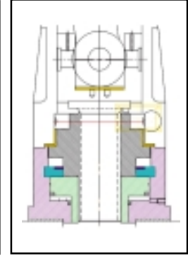
Wrist Pin
