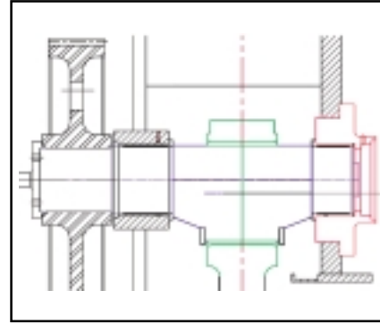
Eccentric Shaft
